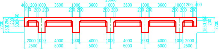
Sect C-C
