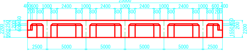
Sect C-C
